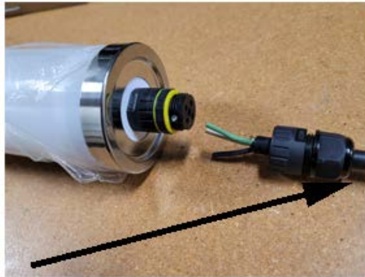
5. Add external power cord (by installer)
