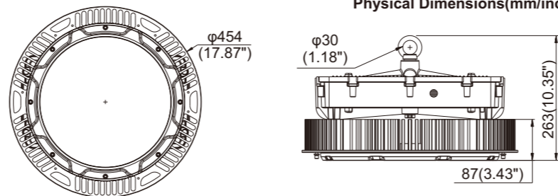
Physical Dimensions(mm/inch)
