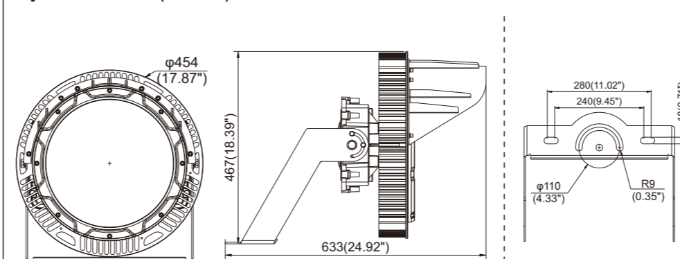
Physical Dimensions(mm/inch)
